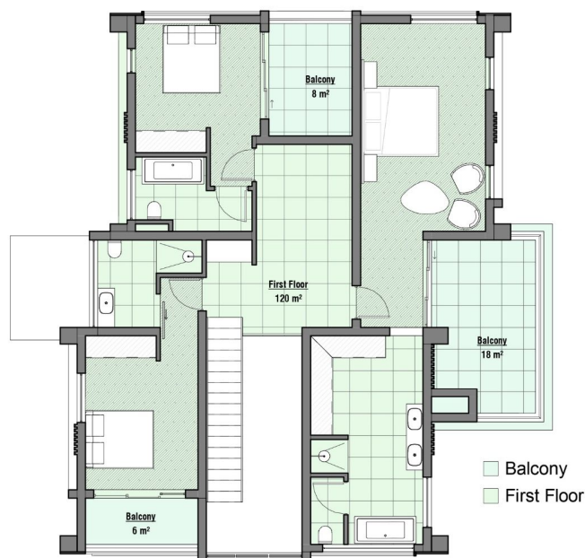
01 First Floor- Area Plan
